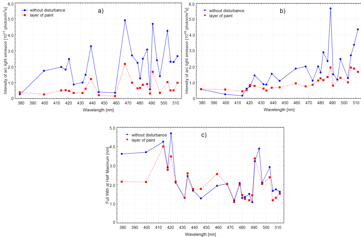
Fig. 12. Influence of paint on the welded plate on the amplitudes (a), the values (b) of additive constant in formula (3), and FWHM (c) of Lorentz functions that best fit the spectral peaks of arc light (welding parameters in text; Attention: curves presented in the figure cannot be interpolated).
