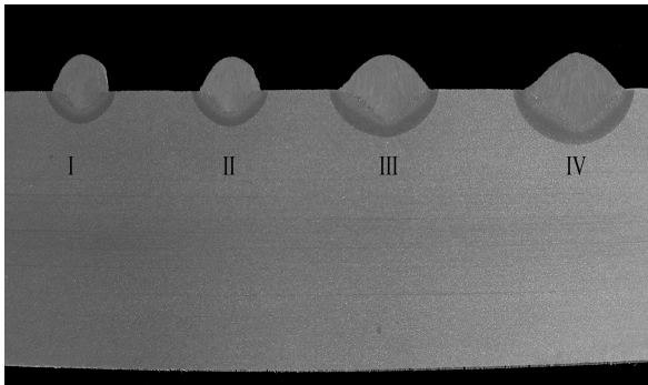
Fig.6. Macroscopic examination of padding welds. Roman numbers represent different beads. The welding parameters are given in Table 2 (etching: Adler; magnification × 1).
