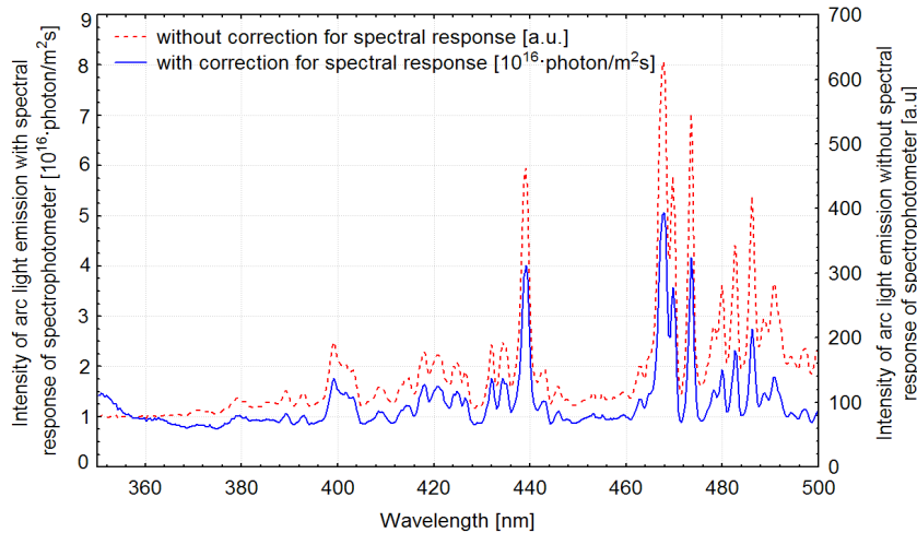
Fig. 4. Influence of sensitivity of spectrophotometer card on the results of measurement of spectrum arc light emission. I=104 A, U=16.5 V, 82% Ar + 18 % CO_2 .
