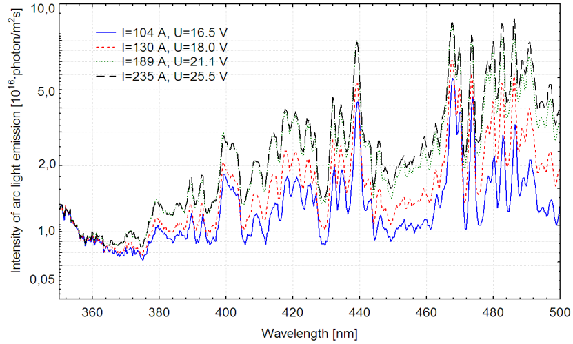
Fig. 7. Effect of the welding current on the arc light spectrum (description of the welding process in the text).
