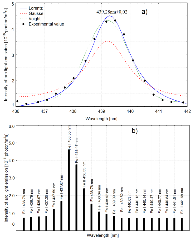
Fig. 8. Comparison of experimental data a) (●) with the best fitted: Gaussian, Lorentz and Voight functions for one of the spectral peaks (from Fig. 7) registered using the CCD device during the welding of clean mild steel S 235 in the Ar + CO 2 shielding gas (Values of the fitted parameters are given in Table 3; I=104 A; U=16.5 V), b) contribution to the observed spectral peak (only Fe and Fe I).
