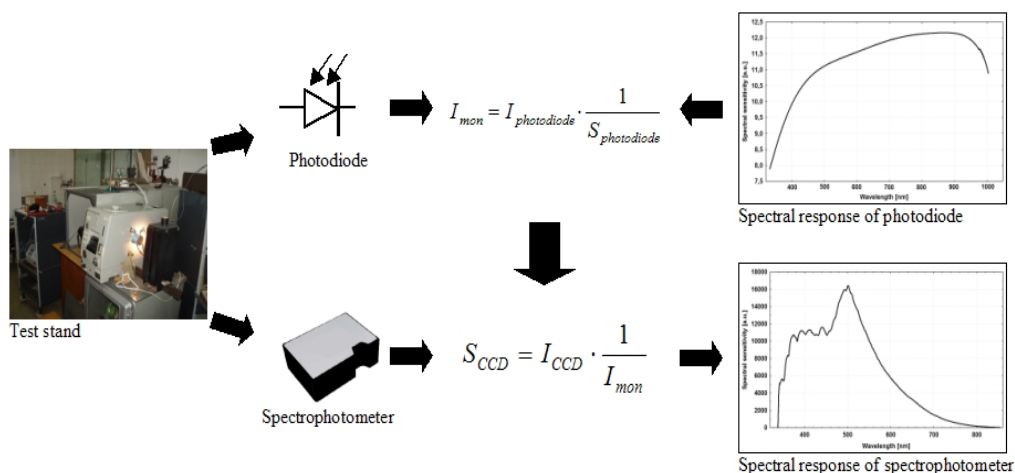
Fig. 3. Methodology to calculate the spectral response characteristic of the spectrophotometer card ( I_{mon} – intensity of light from monochromator [ \text{photon}/(\text{m}^2 \cdot \text{s}) ], I_{photodiode} – density of short-circuit current from the photodiode on the photosensitivity area of the photodiode, S_{photodiode} – sensitivity of photodiode for the appropriate wavelength, I_{CCD} – intensity of light measured in relative units by the spectrophotometer card, S_{CCD} – sensitivity of spectrophotometer card for the appropriate wavelength).
