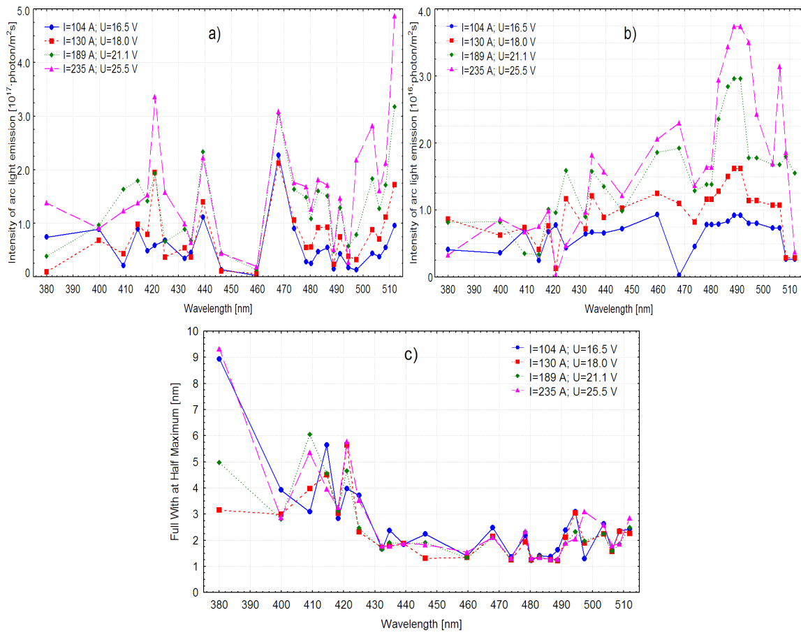
Fig. 9. Influence of welding current intensity on the amplitudes (a), the values (b) of additive constant in formula (3), and FWHM (c) of Lorentz functions that best fit the spectral peaks of arc light (other welding parameters from Table 2. Attention: curves presented in the figure cannot be interpolated).
